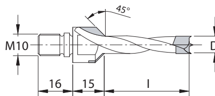
ATTACCO PER MACCHINE/SHANK FOR MACHINES: Biesse, Morbidelli, Masterwood, Weeke, Vitap (new type)
